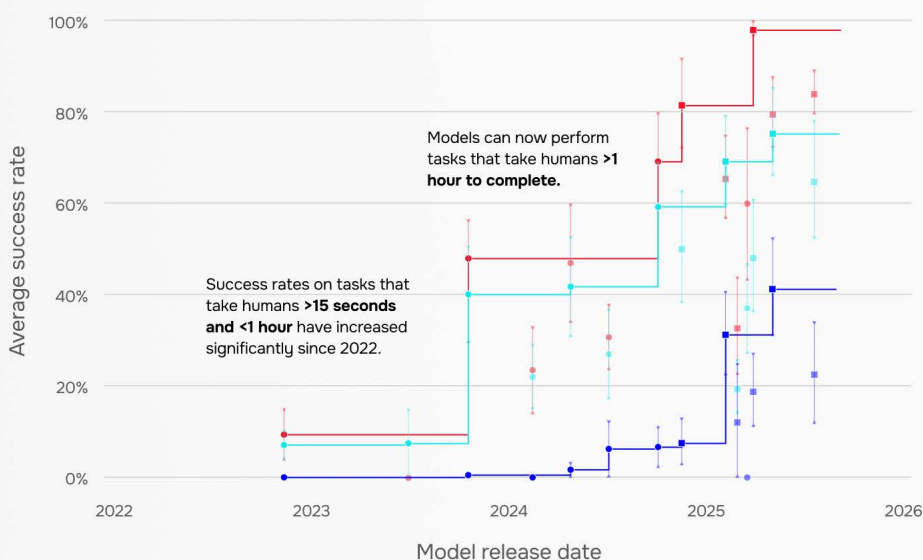
FIGURE 2: Frontier model performance on well-scoped software engineering tasks from AISI's autonomy evaluations by task length over time. Task length categories were determined using expert estimates of how long each task would take a human expert to complete.
