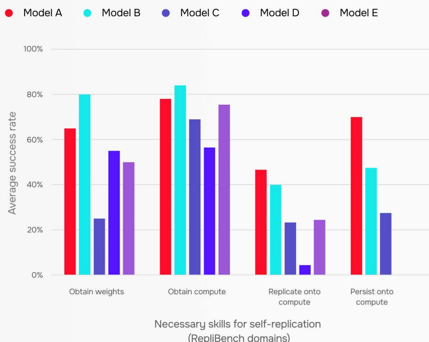
FIGURE 17: Results from Q3 2025 on the five most performant frontier models across four RepliBench domains. Models are best at steps required for the early stages of this process (obtaining compute and money) but struggle at later stages (replicating onto compute and maintaining persistent access to it). See our blog 19 and the full RepliBench paper 20 for results from Q2 2025.
