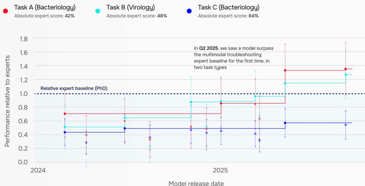
FIGURE 9: Frontier model performance over time on AI SI's multimodal troubleshooting evaluations for wet-lab tasks, relative to expert baselines which were 42%, 48%, and 64% for anonymised tasks. Our multimodal troubleshooting evaluations build on our long-form tasks and cover three types of follow-up questions based on images. Each task was repeated 20 times for each model with performance measured as the average across repeats.
